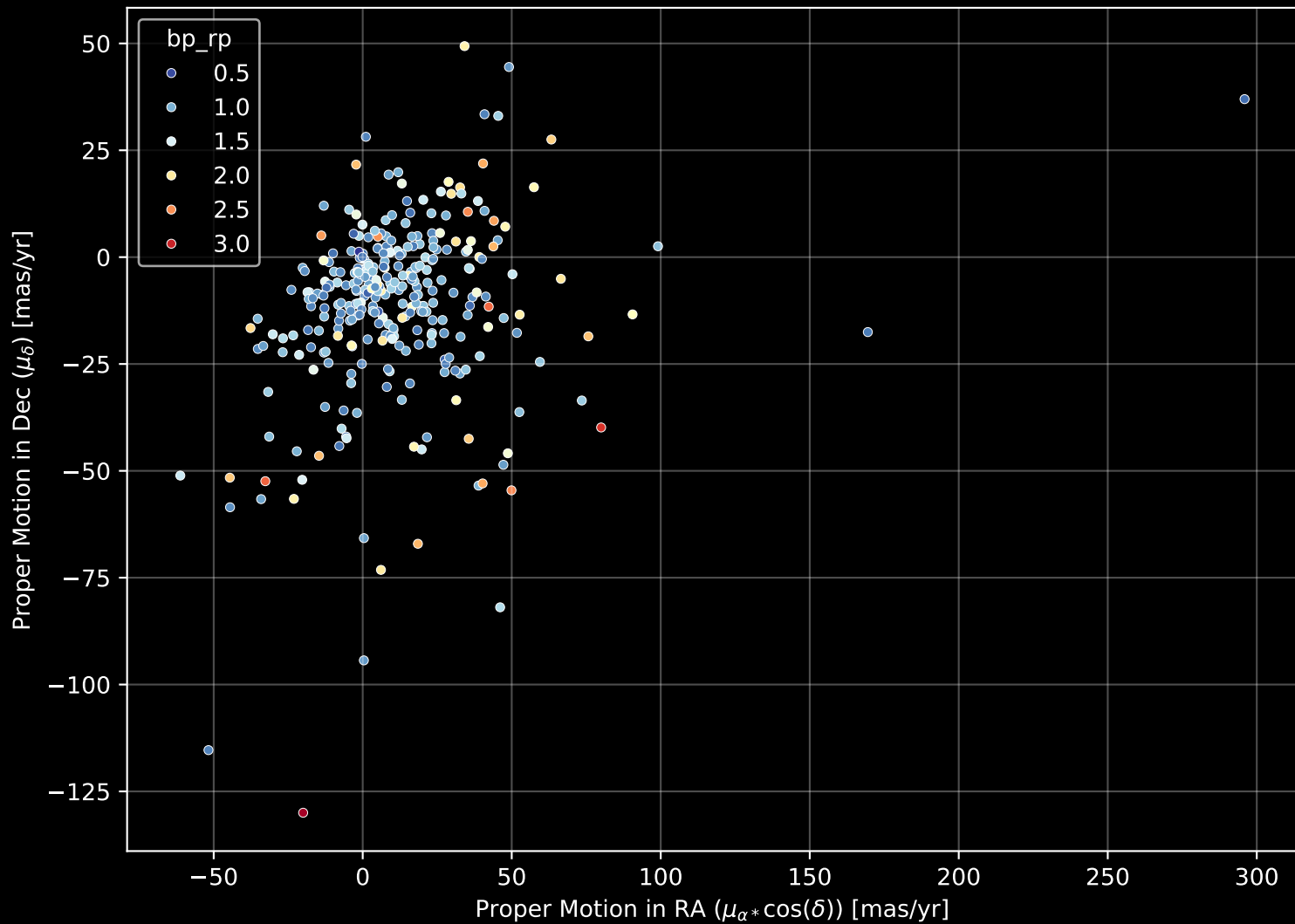
APOGEE DR17 Field: [066-79] Proper Motion Diagram (n= 313)
