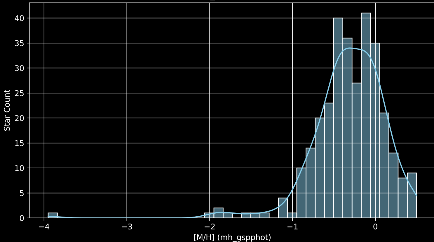
APOGEE DR17 Field: [066-79 [M/H] (mh_gspphot) (n= 310)
