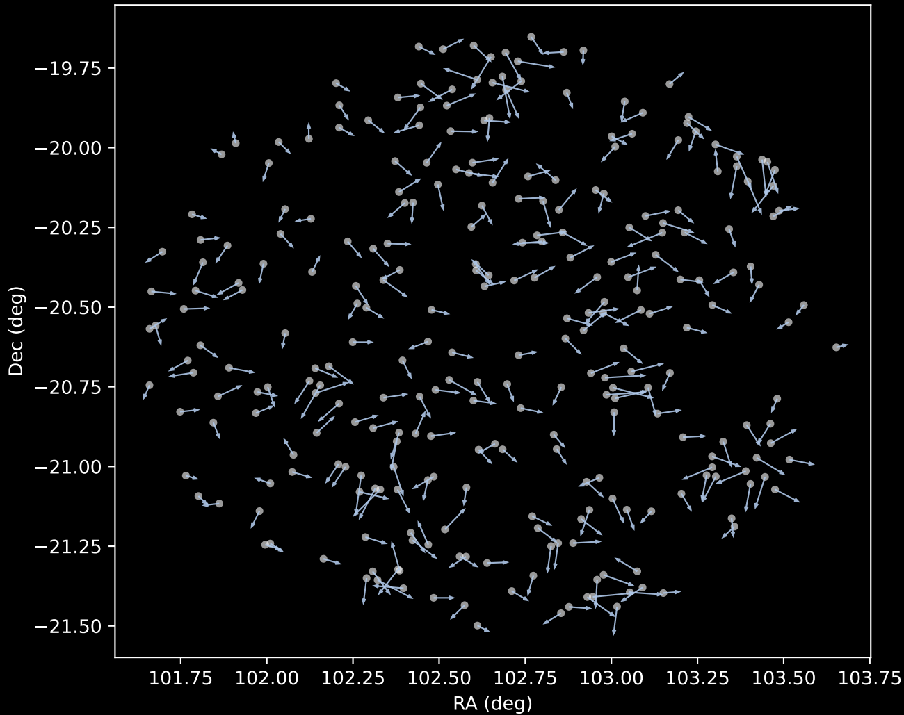
APOGEE DR17 Cluster 1 Proper Motion Vectors (n=277)
