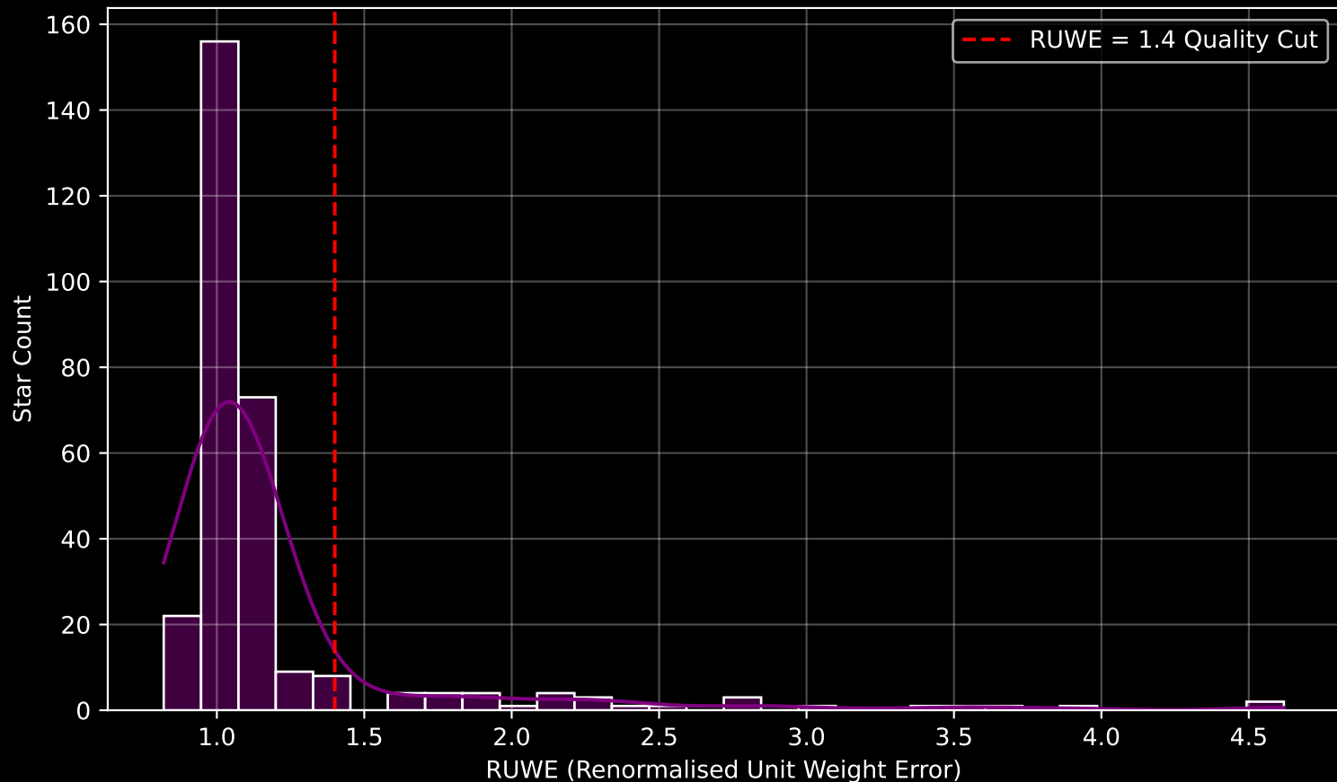
GAPOGEE DR17 Field [066-79] RUWE Distribution (n= 300)
