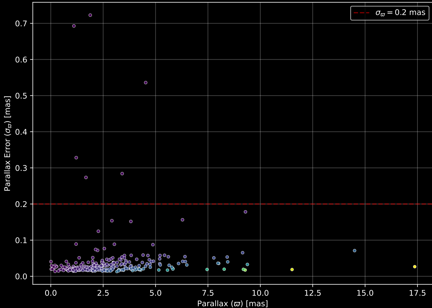
APOGEE DR17 Field: [066-79] Parallax Quality (n= 313)
