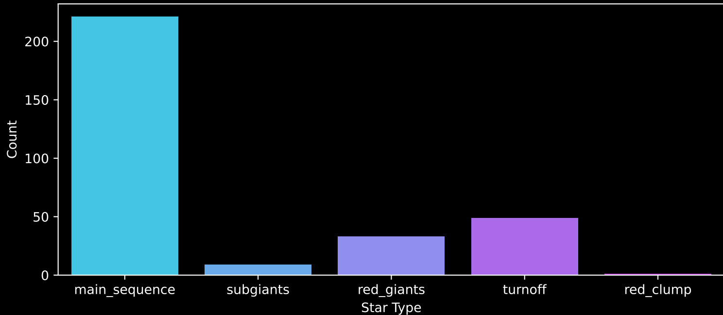
APOGEE DR17 Field: [066-79] Count plot of Star Type
